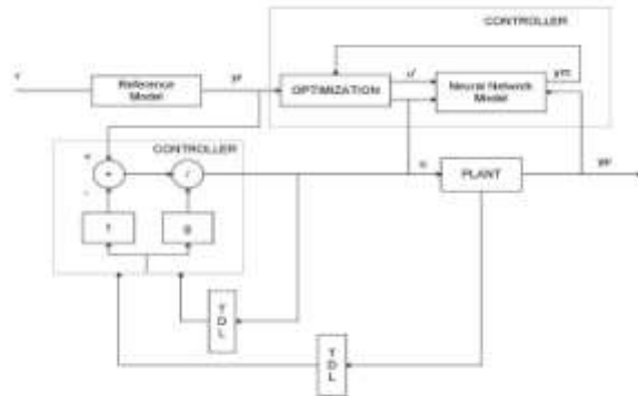
Fig. 7. Block diagram of the model predictive control process
