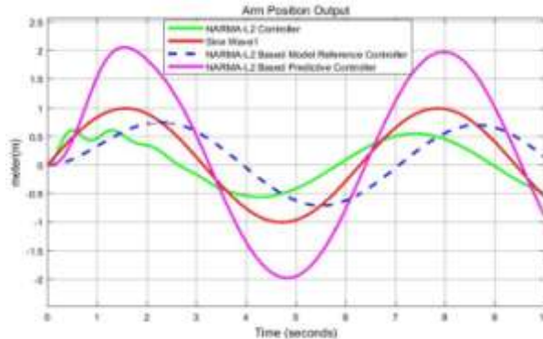
Fig. 13. Sine wave response simulation result
