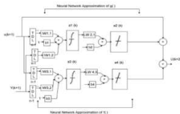
Fig. 2. The structure of a neural network representation.
