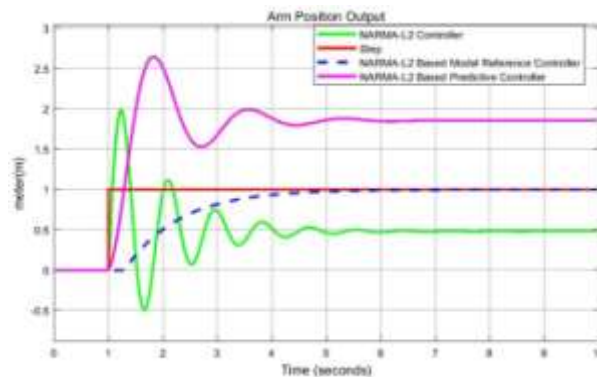
Fig. 11. Step response simulation result
